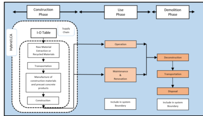
Figure 3. System boundary for LCA in construction process [12]
